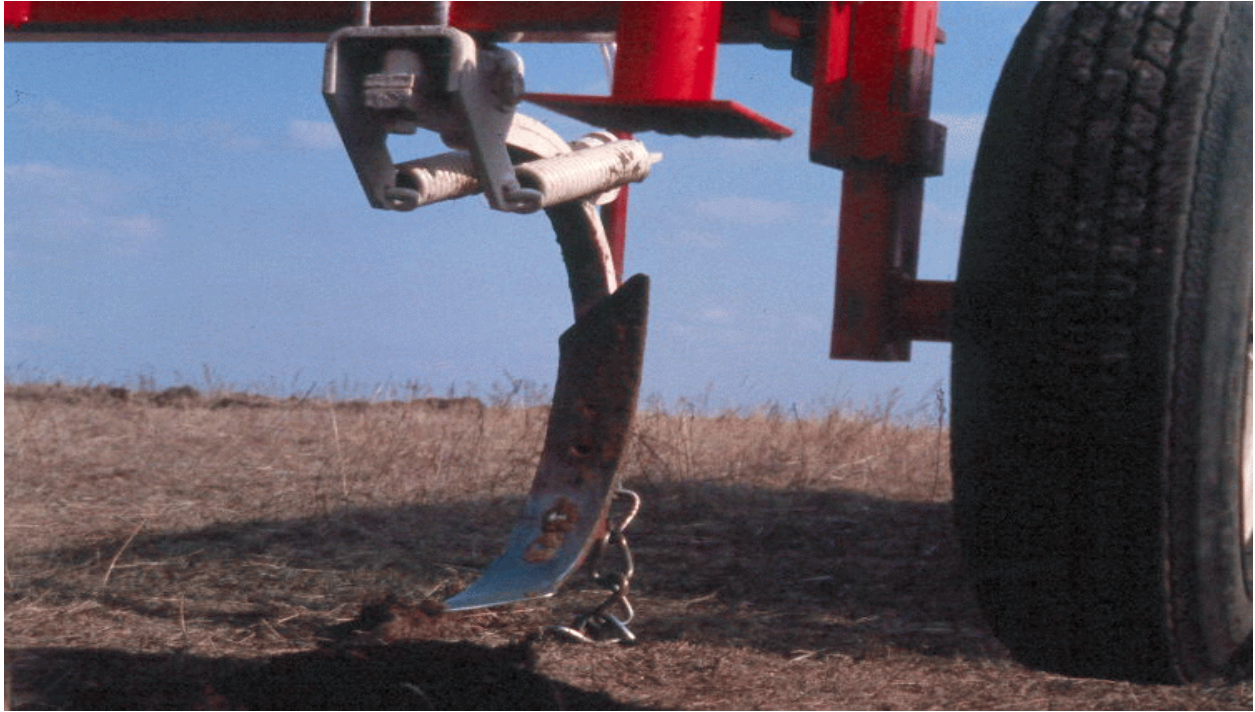
Fig. 5. Four-inch twisted chisel plow shovel.
