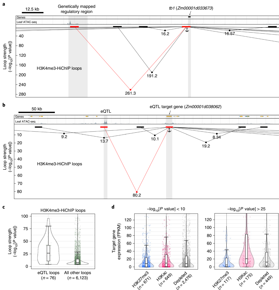
Fig. 4 | Loop strength identifies specific CRE-gene regulatory interactions. a, b , Genome browser shot of tb1 and its fine-mapped distal regulatory region ( a ) and a genetically mapped eQTL and its predicted target gene ( b ). Chromatin loops are represented as line segments with dots indicating -\log_{10}[P] . Black and red blocks represent loop edges for all loops interacting with the tb1 locus (indicated as anchor). The red boxes, connected by red line segments, represent the local loop with the highest contact significance that interacts with the anchor region; the black boxes, connected by black line segments, represent all of the other local loops that interact with the anchor region (that is, not the most significant loop). Panels a and b were not performed in replicate. c , The statistical significance of all H3K4me3-HiChIP loops that link dACR-overlapping eQTL to their target genes versus all other dACR-gene H3K4me3-HiChIP loops. d , The expression of target genes at one edge of the loop and dACR at the other end of the loop, split into the three chromatin groups, as classified in Fig. 2. Shown are loops at high and low -\log_{10}[P] . Boxplots in c and d include a median with quartiles and outliers above the top whiskers. All P values were determined in the FitHiChIP program using a two-tailed binomial test.
